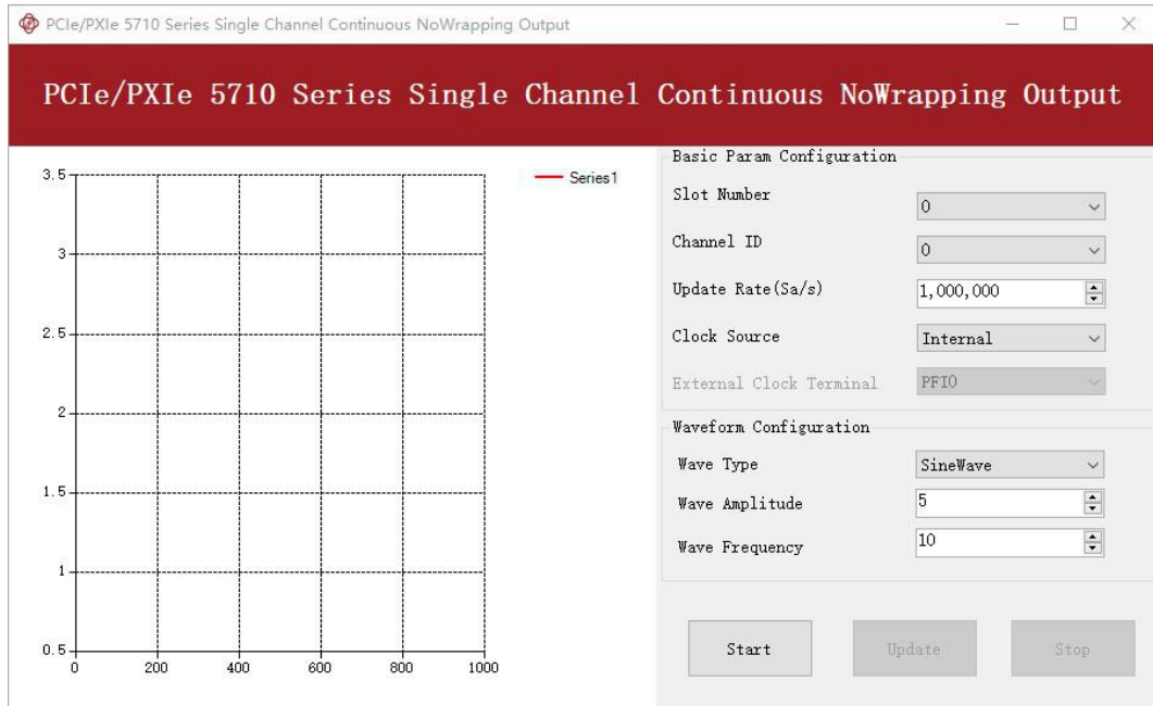
Figure 8 Continuous NoWrapping Output for Single Channel Setting
