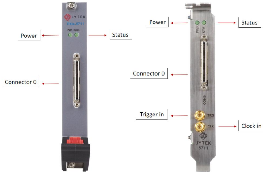
Figure 3 PXIe/PCIe 5710 Front Panel
